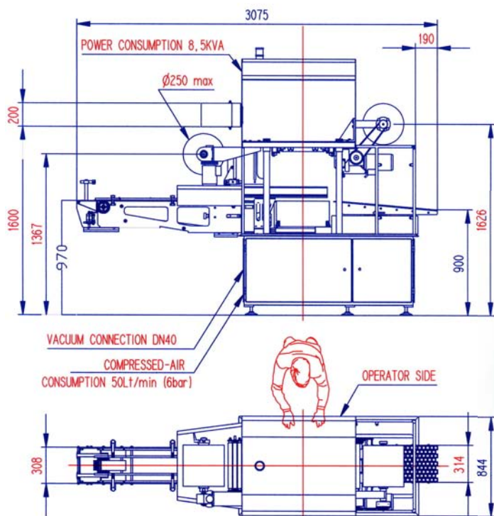
•Machine layout Diagram
